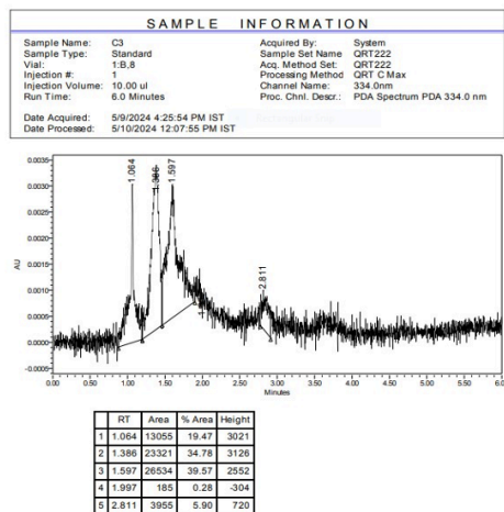
Figure 3 : Analysis Reports
