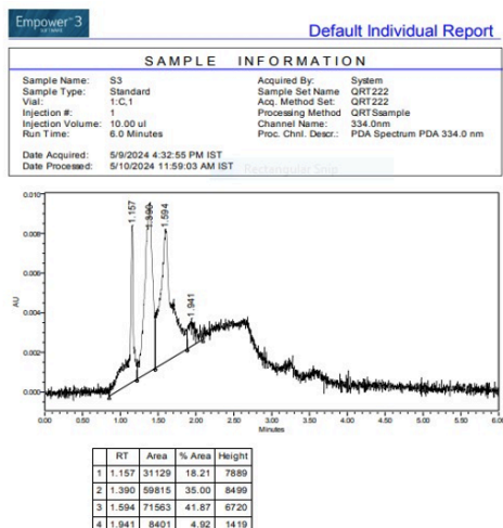
Figure 4: Analysis Reports
