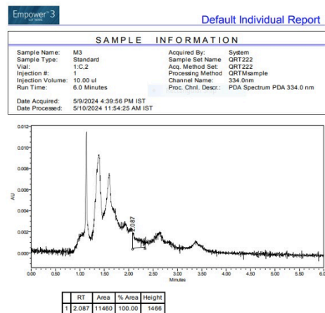
Figure 5 : Analysis Reports
